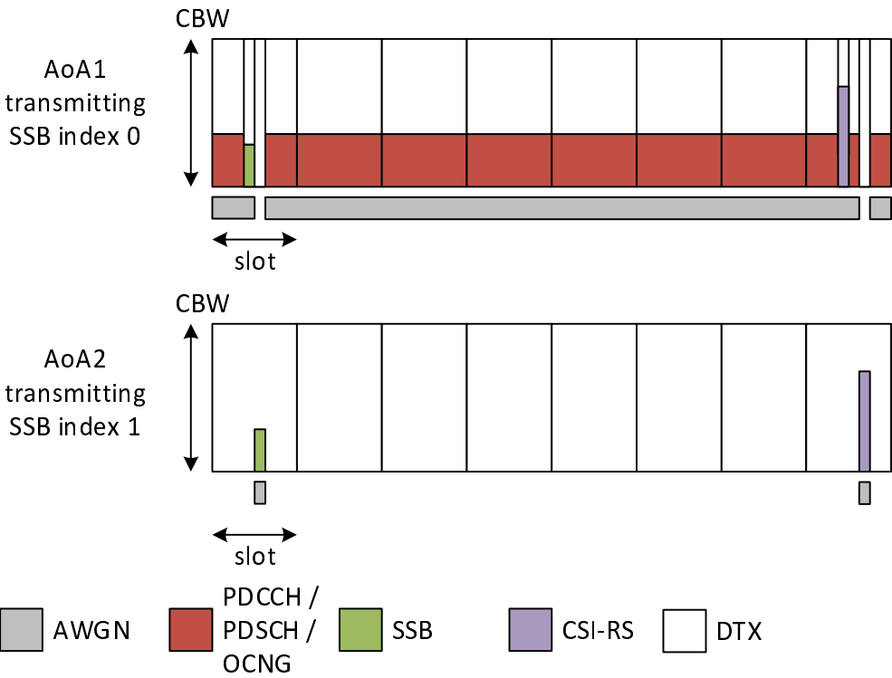
Figure A.5.8.1.1.1-1: Time multiplexed downlink transmissions during T1
