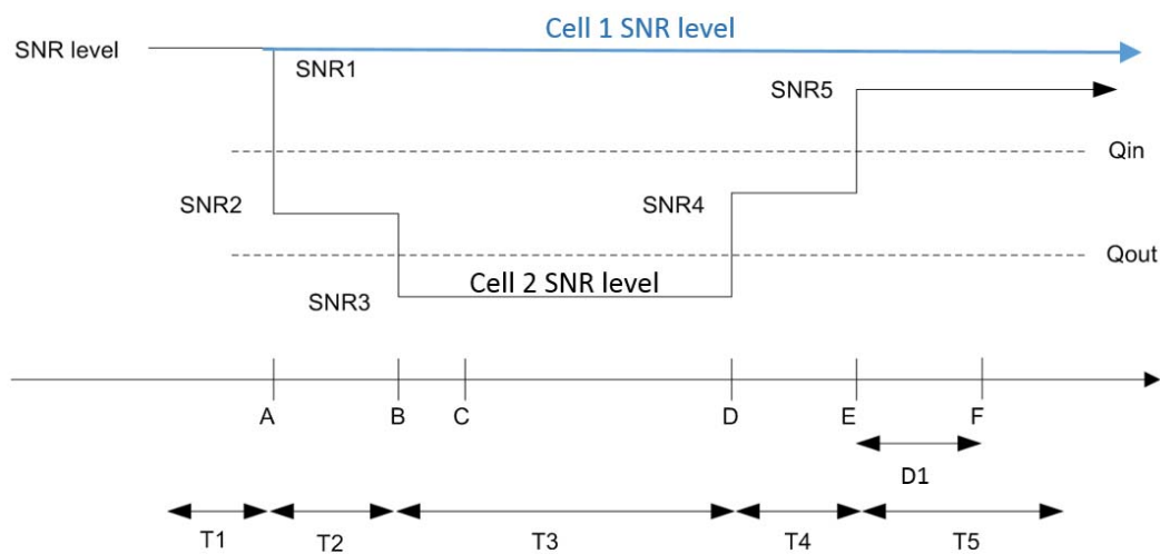
Figure A.4.5.1.4.1-1: SNR variation for in-sync testing
