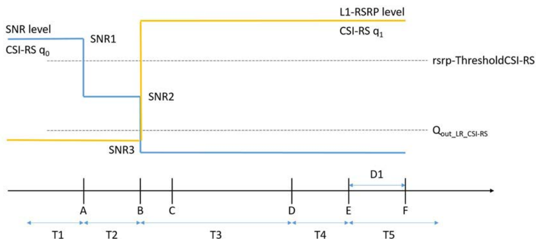
Figure A.7.5.3.1-1: SNR and L1-RSRP variation for CSI-RS based beam failure detection and link recovery testing in non-DRX mode
