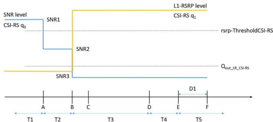
Figure A.5.5.4.1-1: SNR and L1-RSRP variation for CSI-RS-based beam failure detection and link recovery testing in DRX mode
