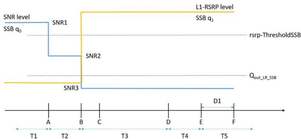
Figure A.5.5.5.1.1-1: SNR and L1-RSRP variation SSB for SSB-based beam failure detection and link recovery testing in non-DRX mode
