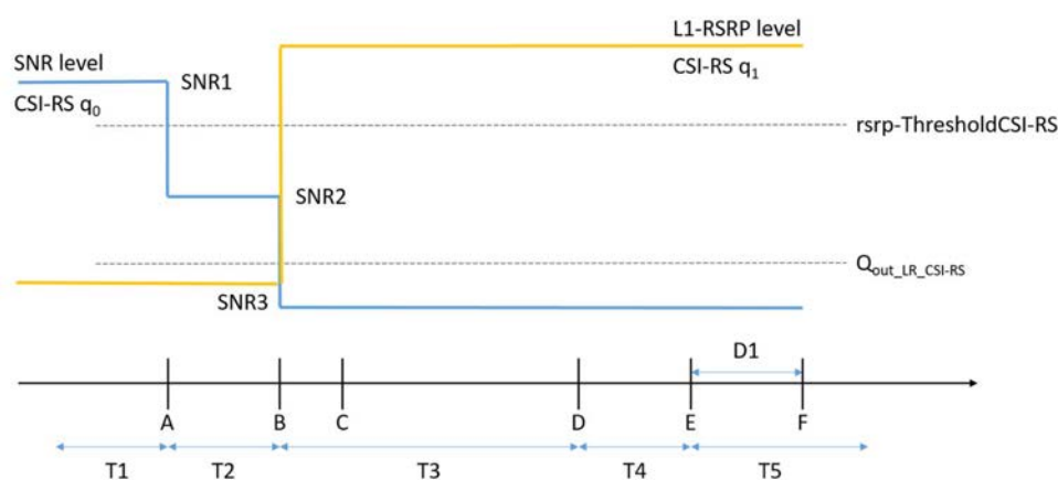
Figure A.5.5.6.1-1: SNR and L1-RSRP variation for CSI-RS based beam failure detection and link recovery testing for SCell in non-DRX mode
