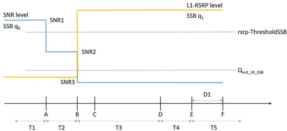
Figure A.10.3.4.1.1-1: SNR and L1-RSRP variation SSB for SSB-based beam failure detection and link recovery testing in non-DRX mode
