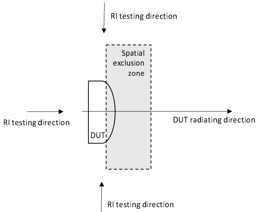
Figure 9.2.2-1: EMC RF electromagnetic field immunity requirement testing directions for 1-O and 2-O BS (horizontal plane depicted)
