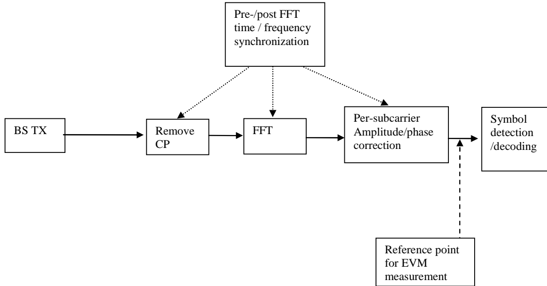
Figure C.1-1: Reference point for EVM measurement
