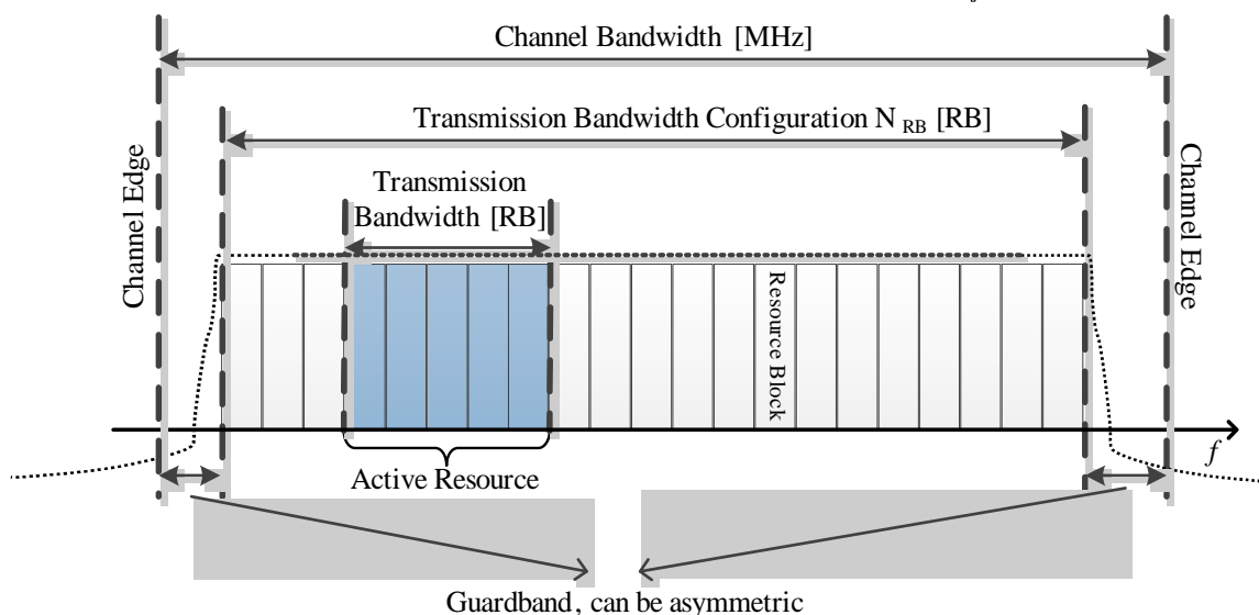
Figure 5.3.3-3 Definition of channel bandwidth and transmission bandwidth configuration for one NR channel
