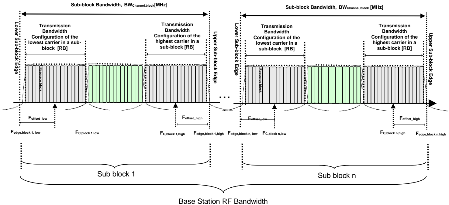
Figure 5.3.3-5 Definition of sub-block bandwidth for intra-band non-contiguous spectrum
