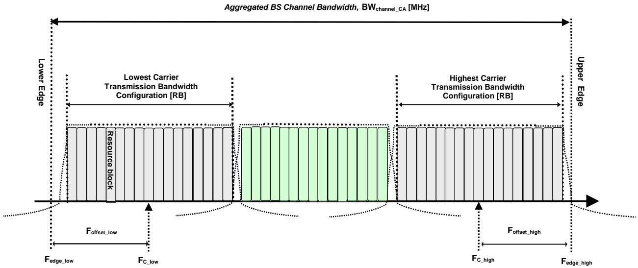
Figure 5.3.3-4 Definition of Aggregated BS Channel Bandwidth for intra-band carrier aggregation
