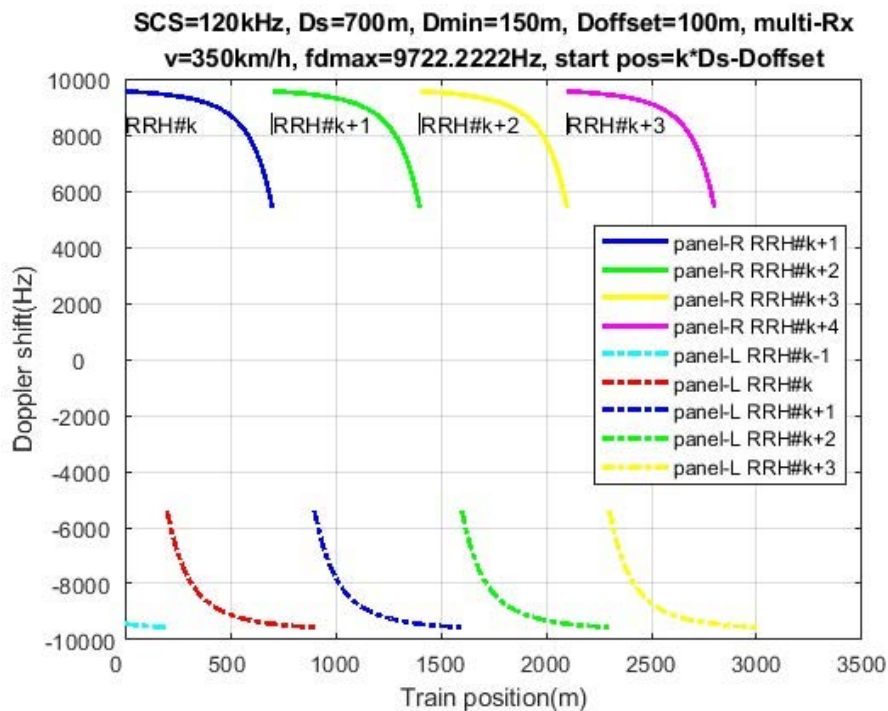
Figure B.3.4.3-3: Doppler shift trajectory ( f_d = 9722 Hz) as seen by PDCCH and PDSCH for each RRH for FR2 HST-DPS Bidirectional scenario with multi-Rx Chain Reception
