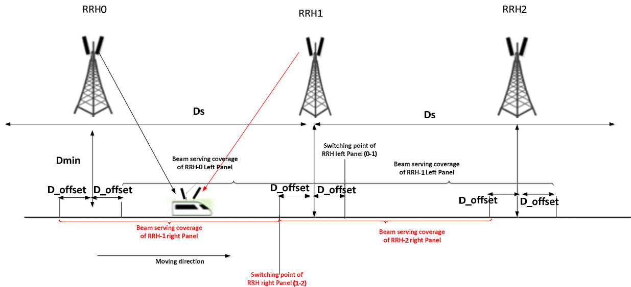
Figure B.3.4.3-1: Bidirectional deployment of FR2 HST-DPS with Multi-Rx Chain Reception
