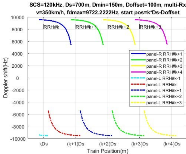
Figure B.3.4.3-2: Doppler shift trajectory ( f_d = 9722 Hz) showing visibility of each RRH for FR2 HST-DPS Bidirectional scenario with mutlit-Rx Chain Reception
