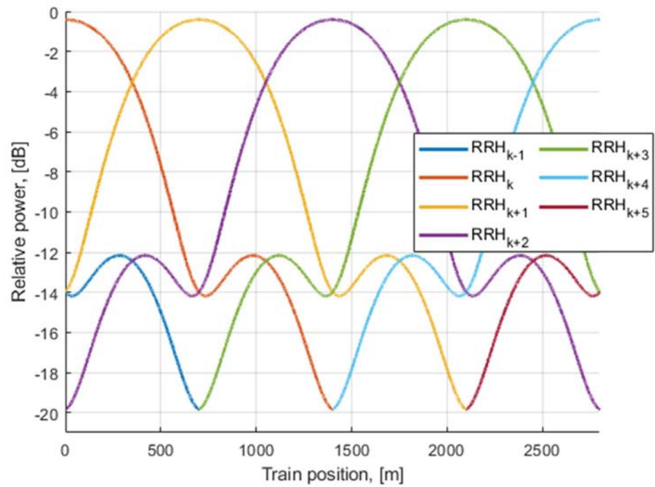
Figure B.3.2-2 Relative power level trajectories
