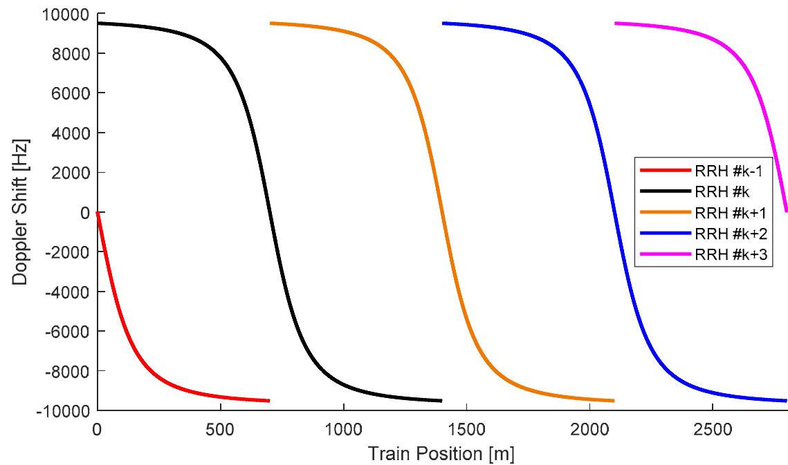
Figure B.3.4.2-2: Doppler shift trajectory ( f_d = 9722 Hz) showing visibility of each RRH for FR2 HST-DPS Bidirectional scenario
