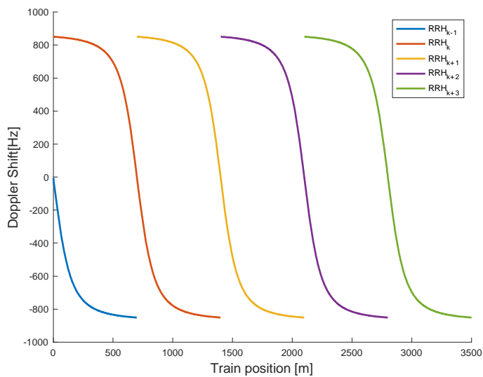
Figure B.3.5-3 Doppler shift trajectory ( f_c = 870 Hz) showing visibility of each RRH
