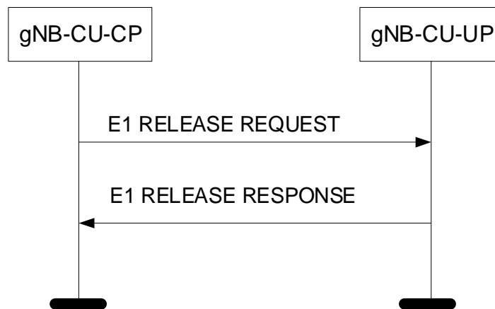
Figure 8.2.7.2.1-1: E1 Release procedure initiated from the gNB-CU-CP. Successful operation.
