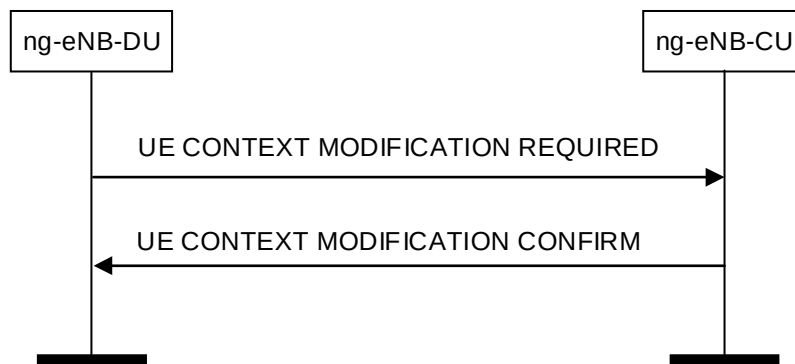
Figure 8.3.5.2-1: UE Context Modification Required procedure. Successful operation
