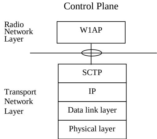
Figure 7.1-1: Interface protocol structure for W1-C
