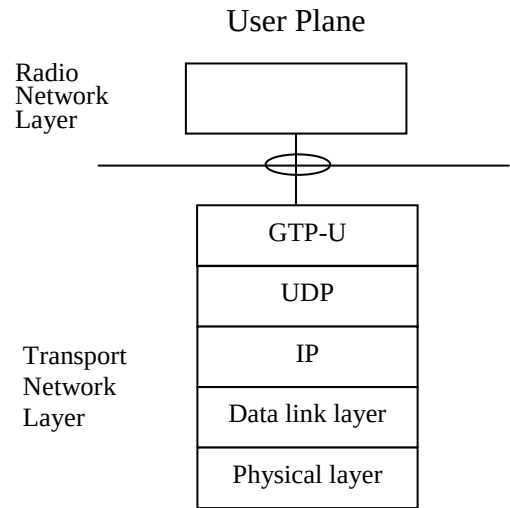
Figure 7.2-1: Interface protocol structure for W1-U
