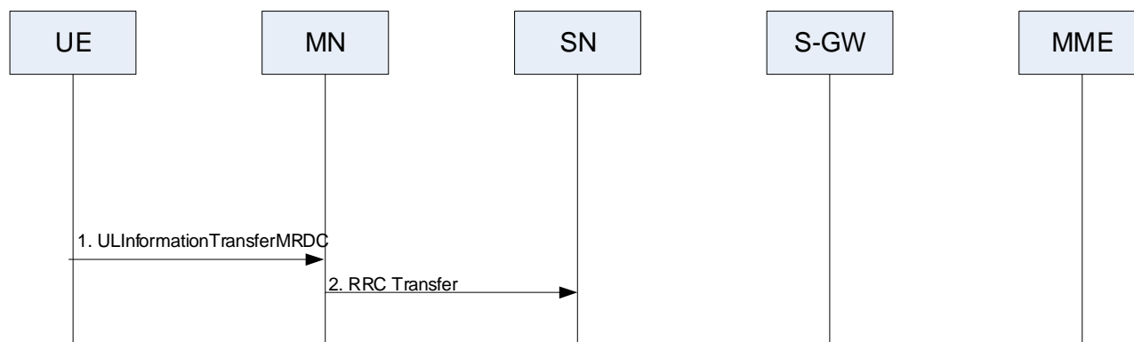
Figure 10.10.1-3: RRC Transfer procedure for NR measurement report, NR failure information, NR UE assistance information or CPC execution completion
