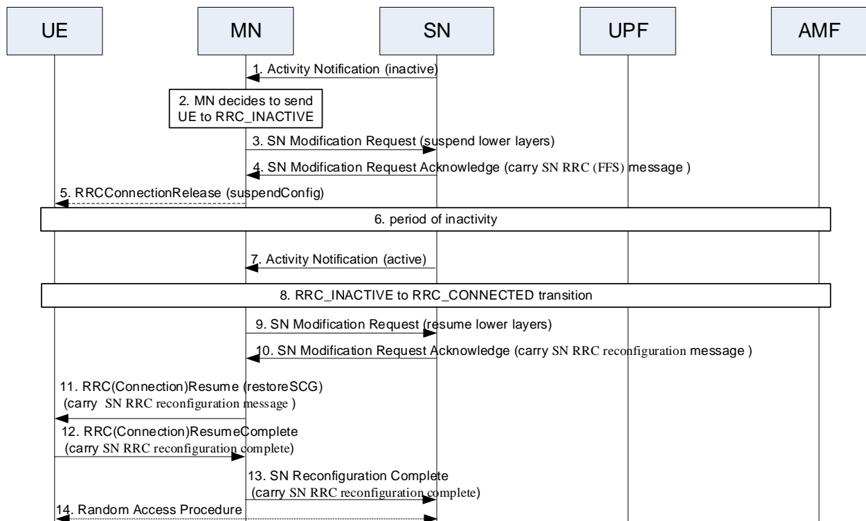
Figure 10.12.2-1: Support of Activity Notification in MR-DC with 5GC with RRC_Inactive - SCG configuration suspended in SN
