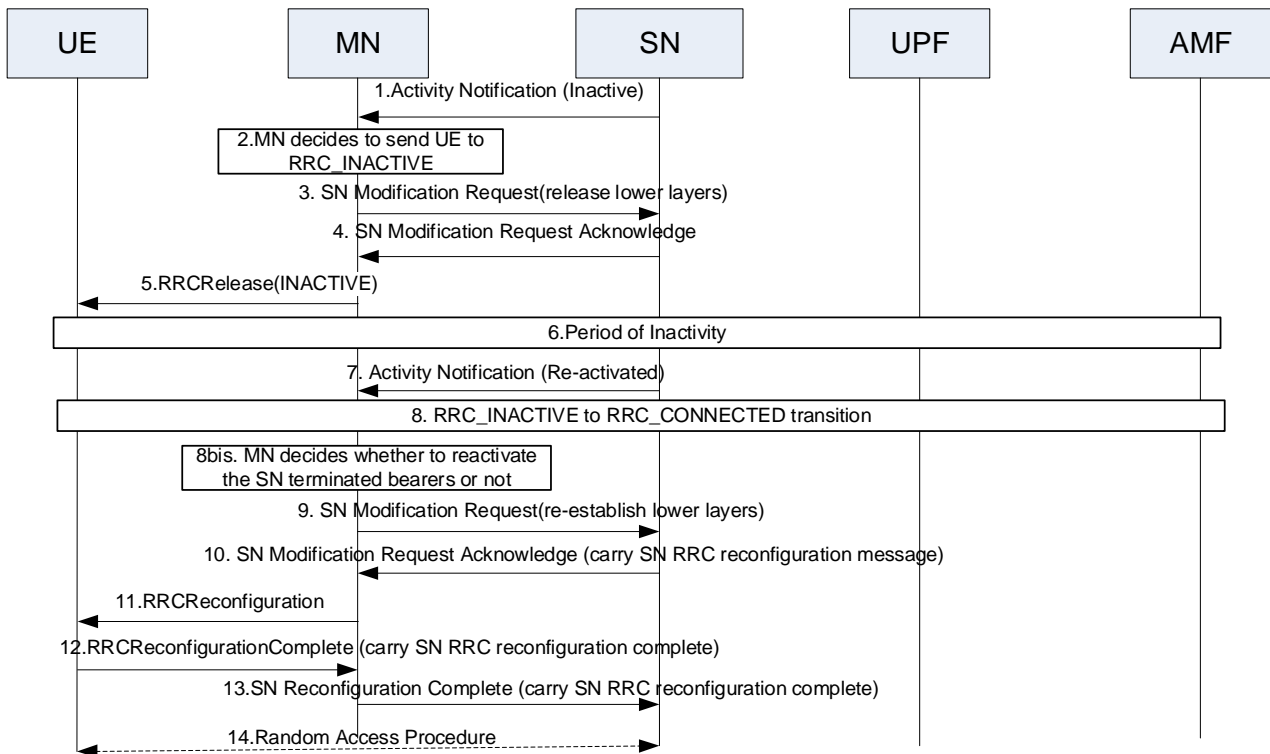
Figure 10.12.2-2: Support of Activity Notification in MR-DC with 5GC with RRC_Inactive – SCG configuration released in SN
