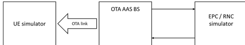
Figure 9.1-2: Communication link set up for OTA AAS BS immunity measurement
