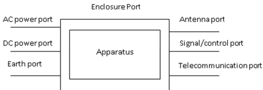
Figure 3.1-1: Examples of ports for hybrid AAS BS
