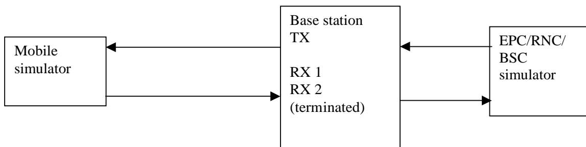
Figure 9.1-1: Communication link set up for BS immunity measurement
