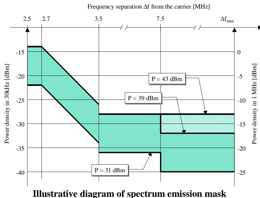
Figure 6.6.4.3.2-1: Spectrum emission mask
