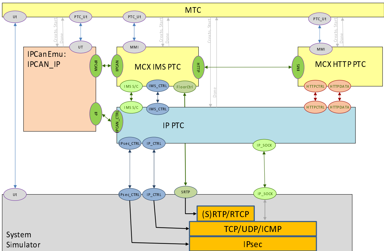
Figure 5.2.1-1: MCX Client on-network test model over IP
