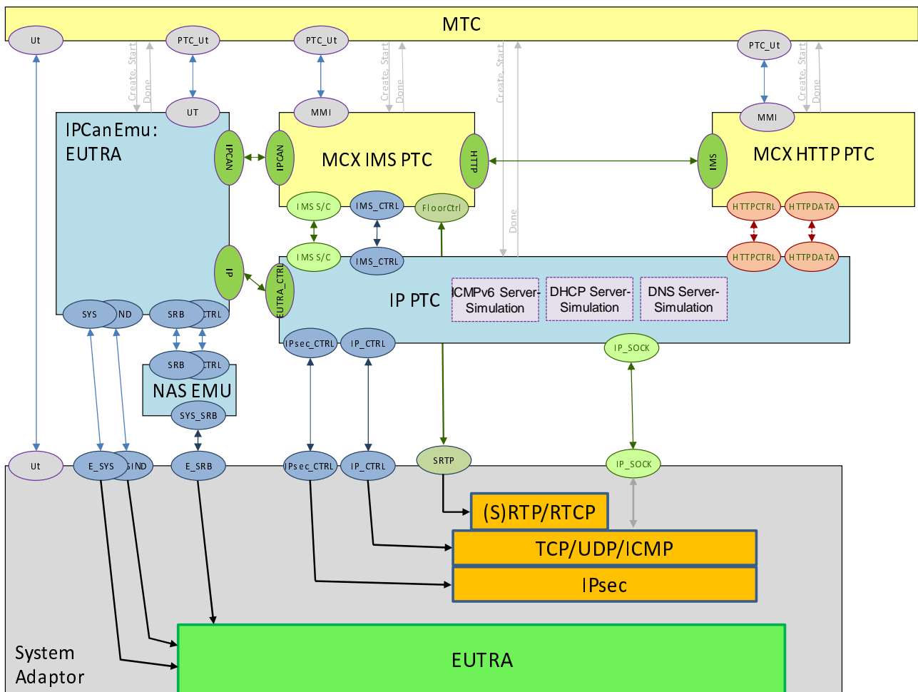
Figure 5.1.1-1: MCX Client on-network test model over LTE
