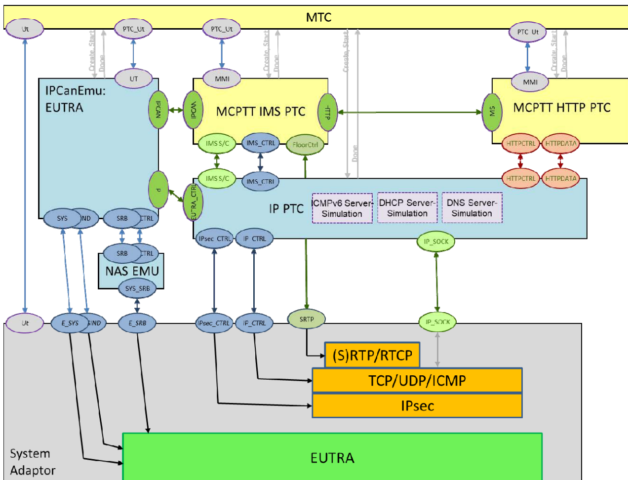
Figure 5.1.1-1: MCPTT Client on-network test model
