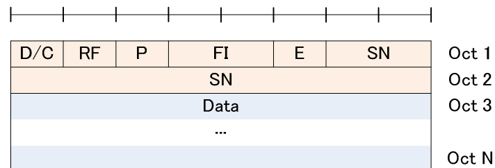
Figure 6.2.1.4-1: AMD PDU with 10 bit SN (length of LI field is 11 bits) (No LI)
