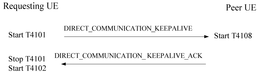
Figure 10.4.3.2.1: Direct link keepalive procedure
