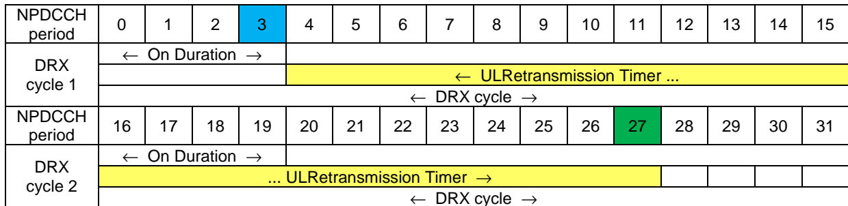
Figure 22.3.1.5.3.2-3: Timing for TP4
