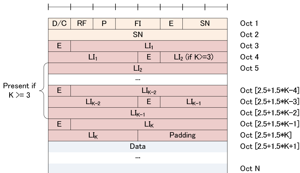
Figure 6.2.1.4-2: AMD PDU with 10 bit SN (length of LI field is 11 bits) (Odd number of LIs, i.e. K = 1, 3, 5, \dots )
