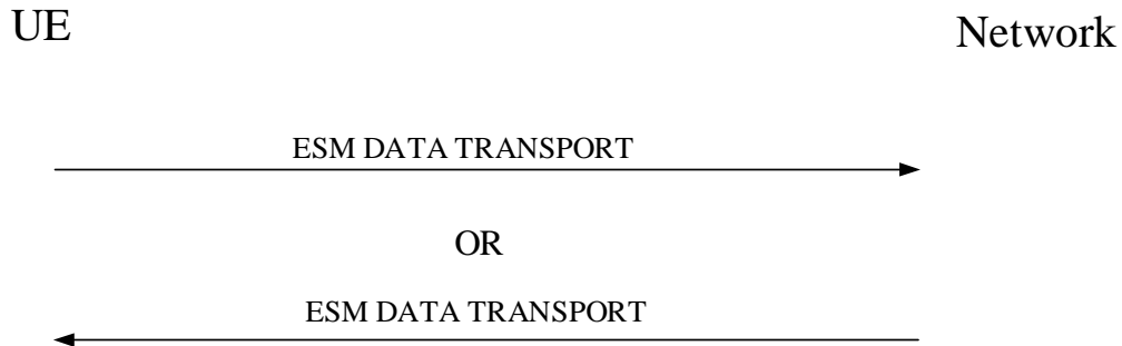
Figure 6.6.4.2.1: Transport of user data via the control plane procedure
