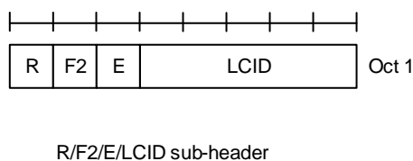
Figure 6.1.2-2: R/F2/E/LCID MAC subheader
