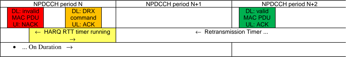
Figure 22.3.1.5.3.2-4: Timing for TP6
