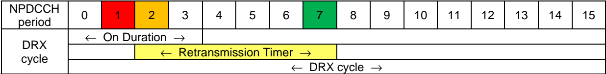
Figure 22.3.1.5.3.2-5: Timing for TP7
