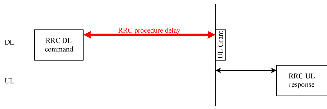
Figure 11.2-1: Illustration of RRC procedure delay
