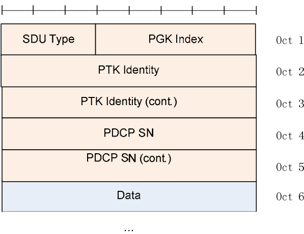
Figure 6.2.10.1: PDCP Data PDU format for SLRB
