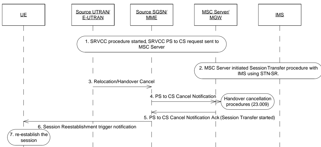
Figure 8.1.3-1: SRVCC Handover Cancellation Procedure
