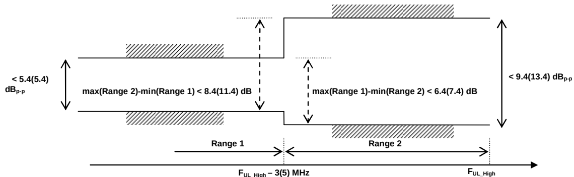
Figure 6.4A.2.4.5-1: The limits for EVM equalizer spectrum flatness with the maximum allowed variation of the coefficients indicated (the ETC minimum requirement within brackets)
