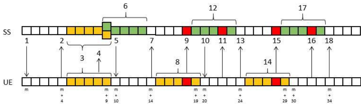
Figure 8.16.58.5-3: Procedure derivation for Activation (The case where the band relation between PCC and SCell1 is intra-band, SCell2 and SCell3 is inter-band)
