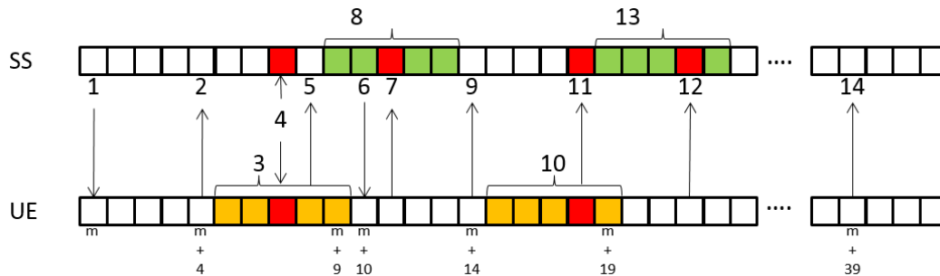
Figure 8.16.39.5-1: Procedure derivation for Activation (the case where the band relation between PCC and SCells are inter-band)
