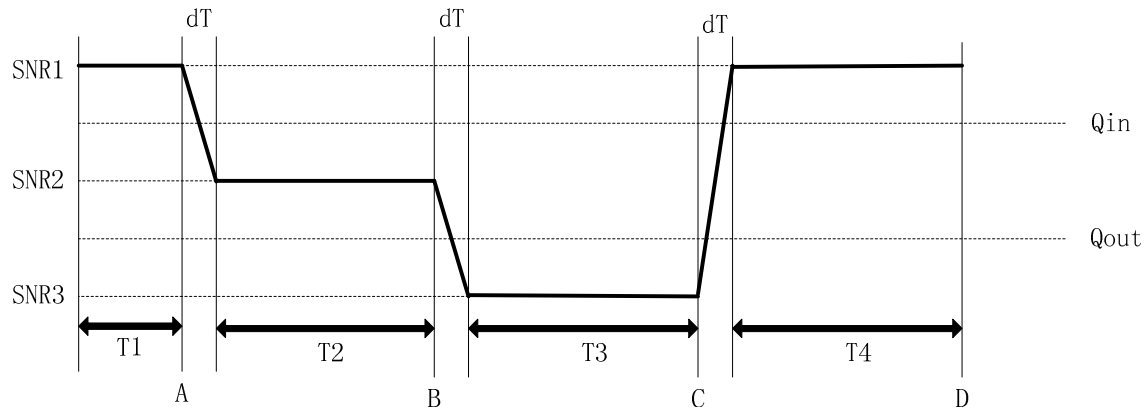
Figure 7.3.60.4-1: SNR variation for out-of-sync testing in DRX for NB-IoT HD-FDD out-of-sync testing for UE category NB1 configured under normal coverage
