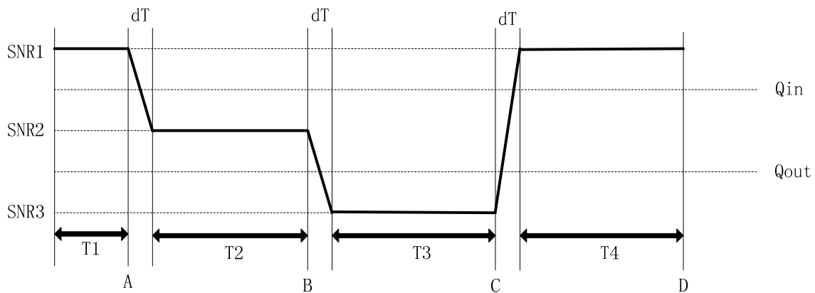
Figure 7.3.61.4-1: SNR variation for out-of-sync testing in DRX for NB-IoT HD-FDD out-of-sync testing for UE category NB1 configured under enhanced coverage
