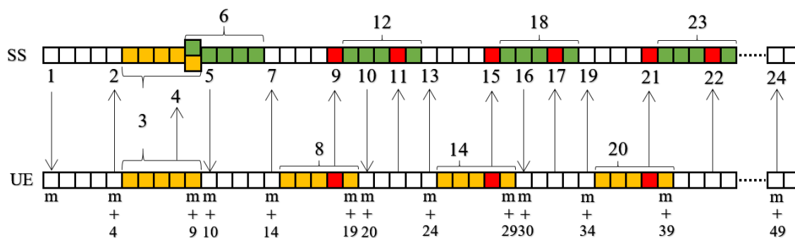
Figure 8.16.69.5-3: Procedure derivation for Activation (The case where the band relation between PCC and SCell1 is intra-band, SCell2, SCell3 and SCell4 is inter-band)
