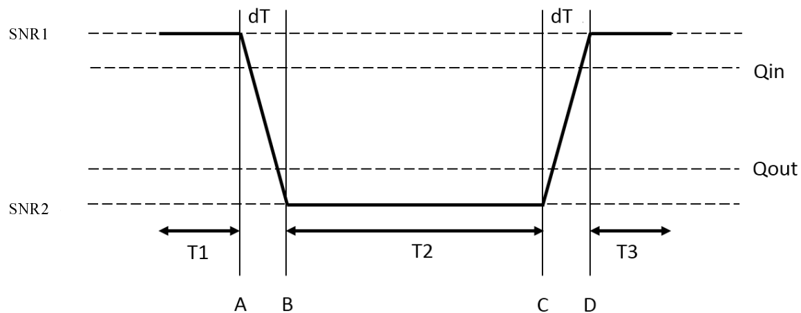
Figure 7.3.62.4-1: SNR variation for in-sync testing with DRX
