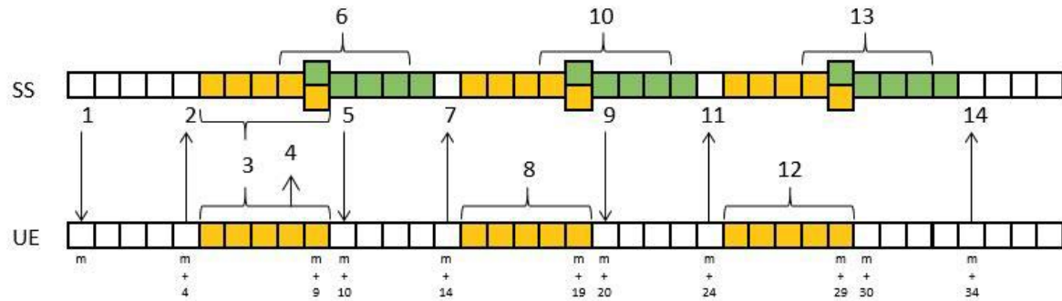
Figure 8.16.58.5-1: Procedure derivation for Activation (All intra-band case)
