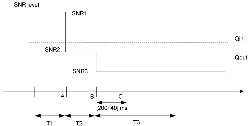
Figure 7.3.18.4-1: SNR variation in the serving cell for out-of-sync testing under time domain measurement resource restriction with CRS assistance information and non-MBSFN ABS
