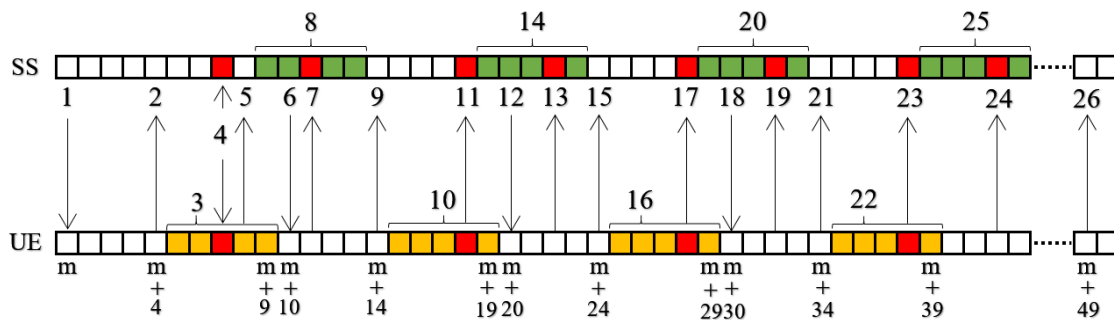
Figure 8.16.67.5-1 Procedure derivation for Activation (the case where the band relation between PCC and SCells are inter-band)
