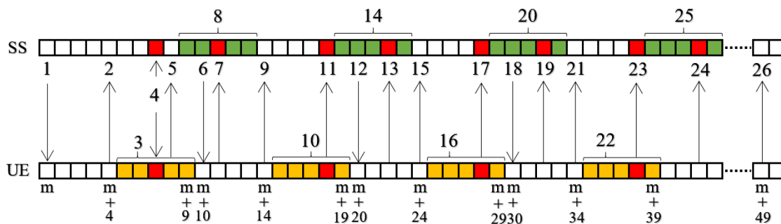
Figure 8.16.69.5-2 Procedure derivation for Activation (the case where the band relation between PCC and SCells are inter-band)
