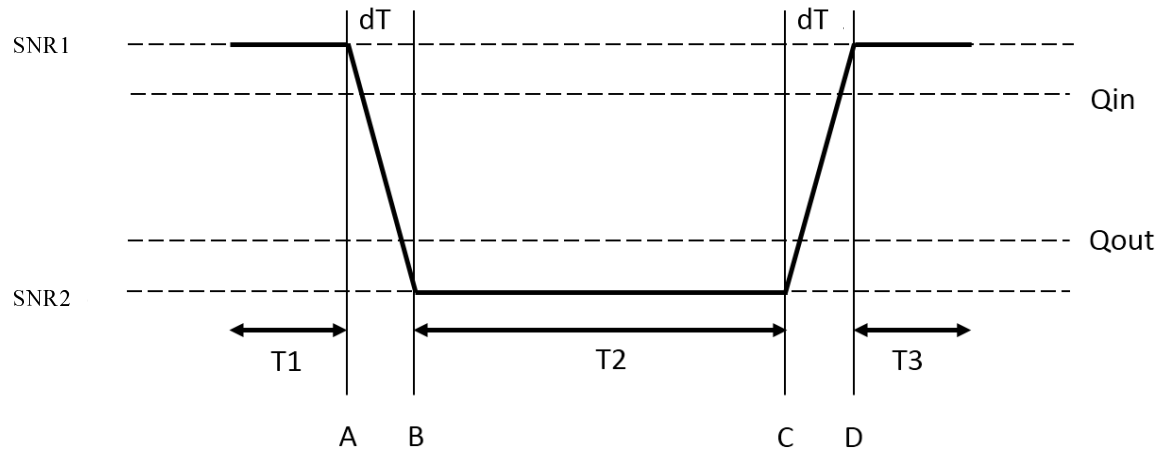
Figure 7.3.64.4-1: SNR variation for in-sync testing without DRX
