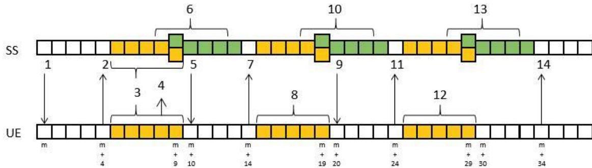
Figure 8.16.57.5-1: Procedure derivation for Activation (All intra-band case)
