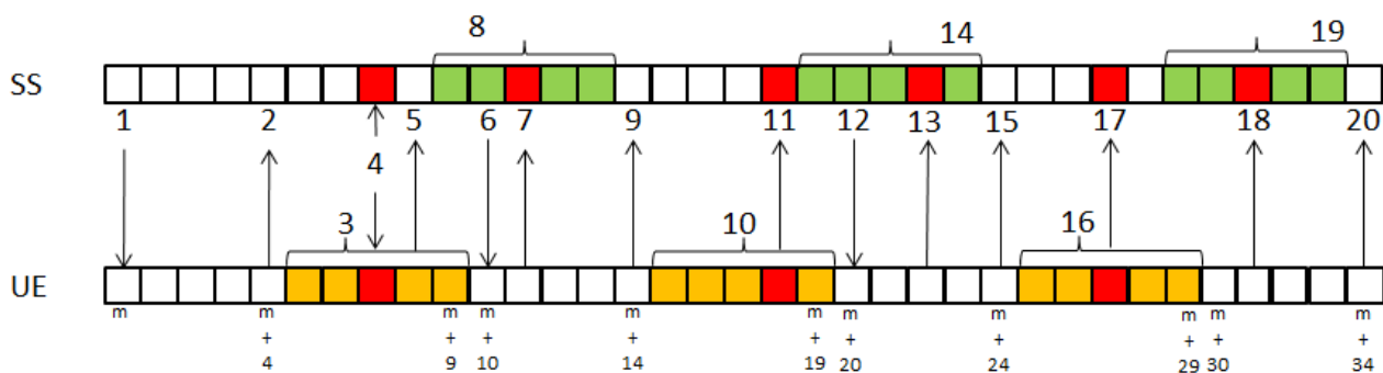
Figure: 8.16.59.5-1 Procedure derivation for Activation (the case where the band relation between PCC and SCells are inter-band)
