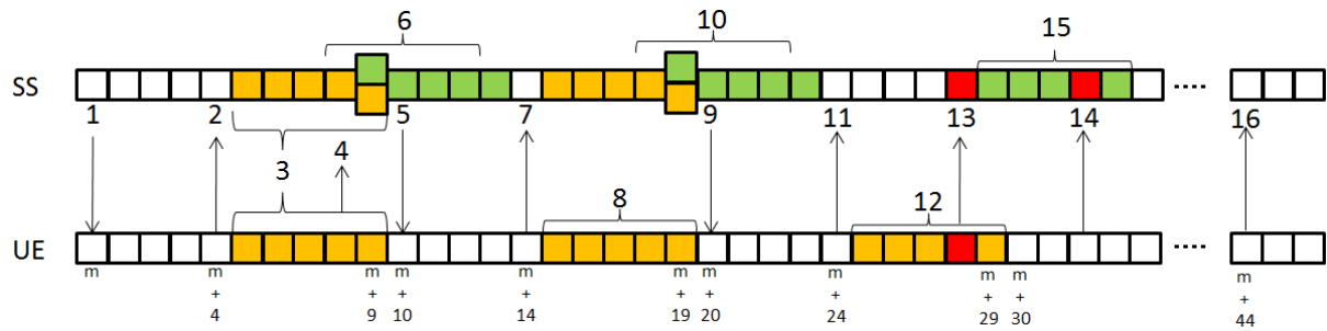
Figure 8.16.61.5-4: Procedure derivation for Activation (The case where the band relation between PCC, SCell1 and SCell2 is intra-band, SCell3 is inter-band)
