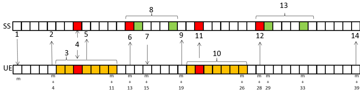
Figure 8.16.36.5-1: Procedure derivation for Activation (the case where the band relation between PCC and SCells are inter-band)
