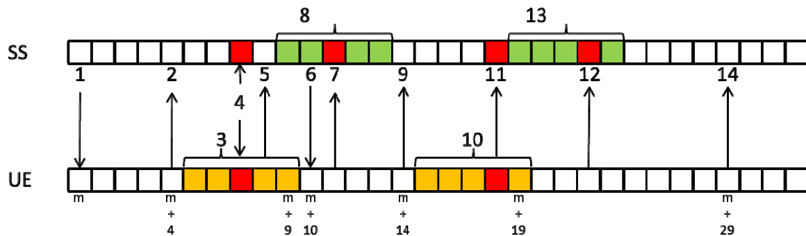
Figure: 8.16.60.5-1 Procedure derivation for Activation (the case where the band relation between PCC and SCells are inter-band)
