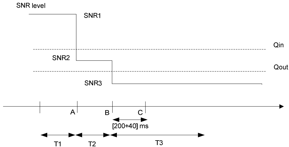
Figure 7.3.17.4-1: SNR variation in the serving cell for out-of-sync testing under time domain measurement resource restriction with CRS assistance information and non-MBSFN ABS
