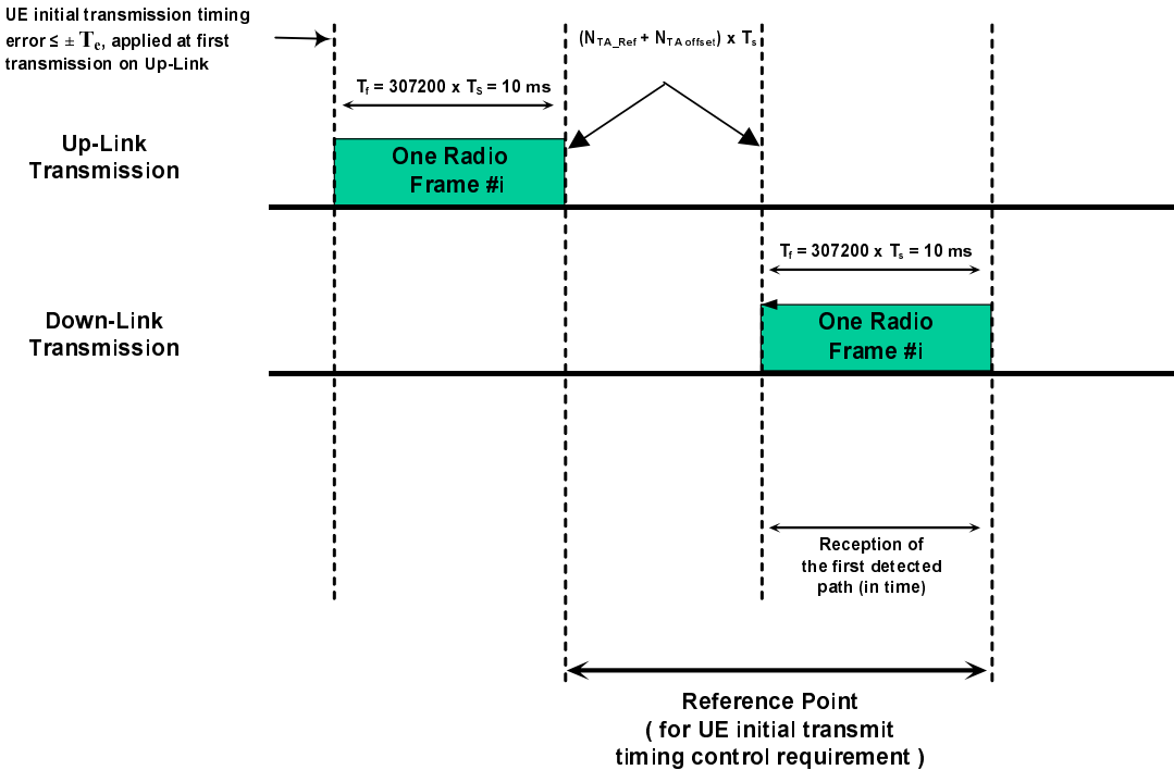
Figure 7.1.1.5-1: Illustration of measurement principle
