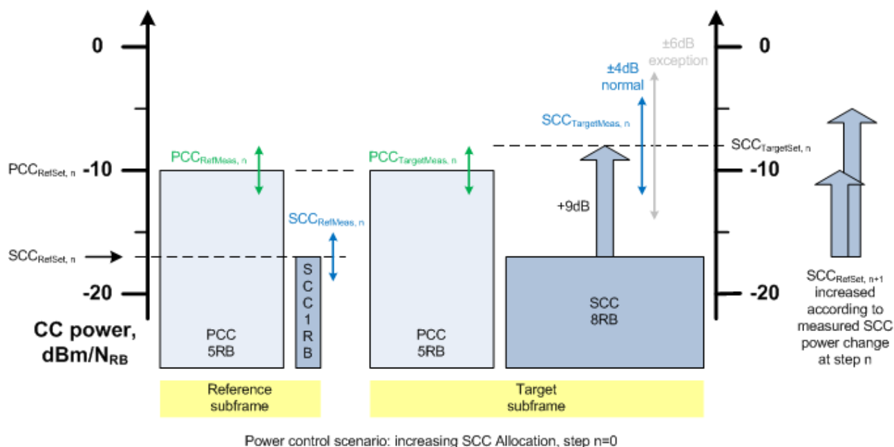
Figure 6.3.5A.2.1.4.2-1: SCC power increase
