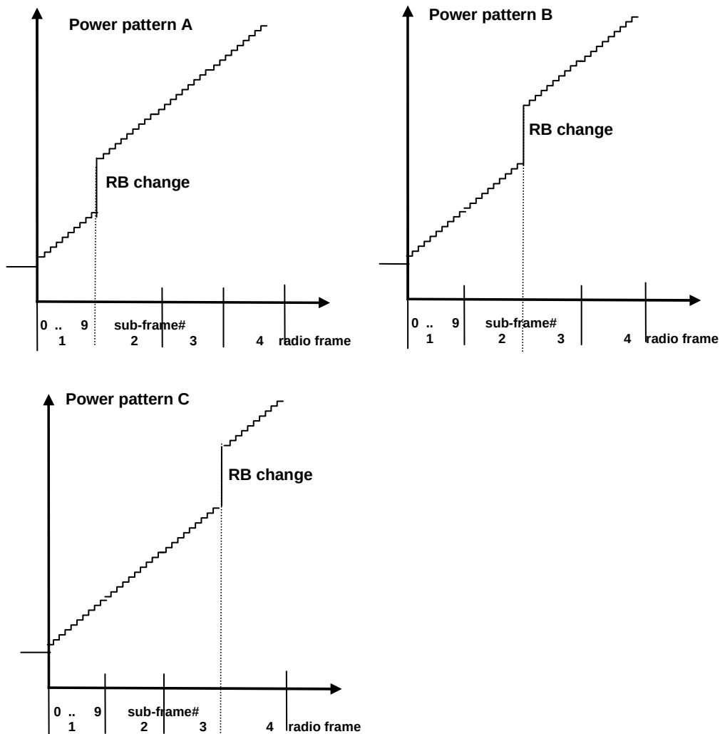
Figure 6.3.5B.2.4.2-1: FDD ramping up test power patterns
