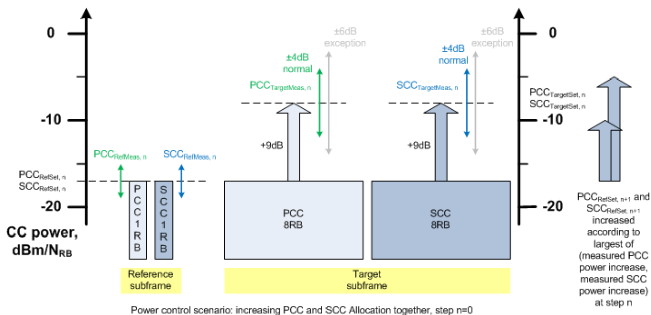
Figure 6.3.5A.2.1.4.2-3: PCC and SCC power increase together
