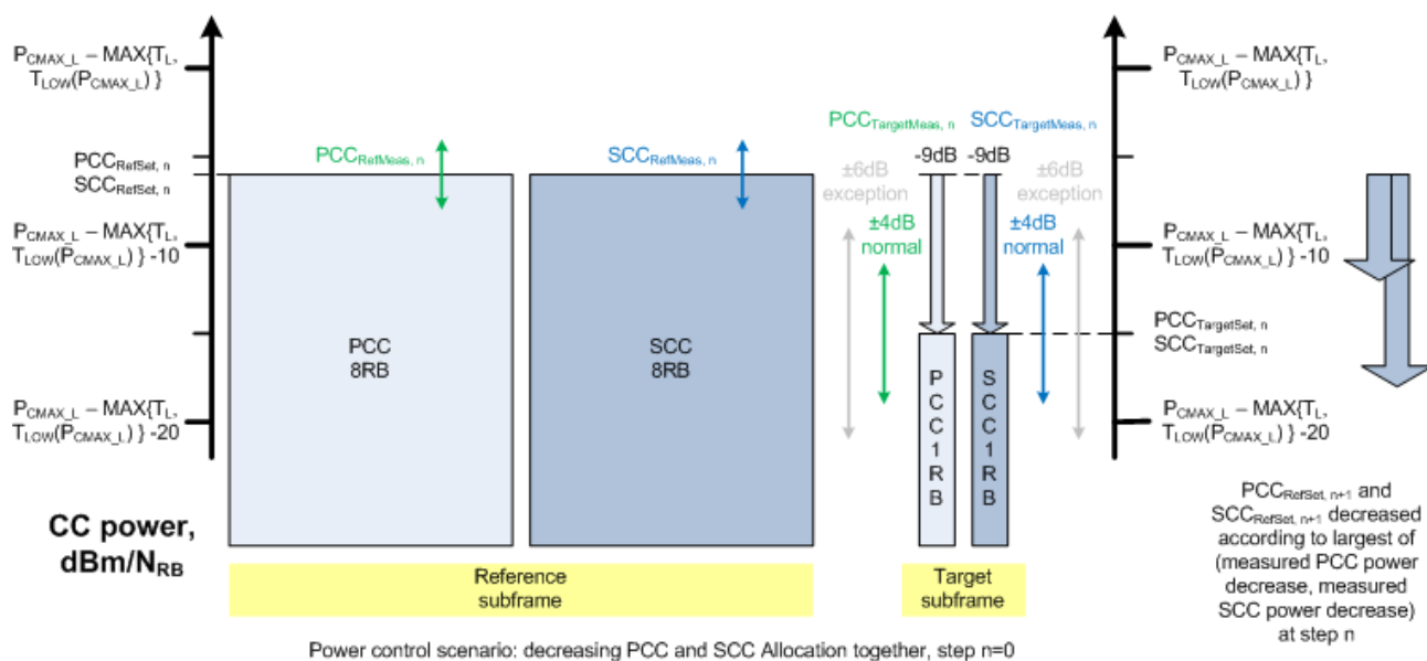
Figure 6.3.5A.2.1.4.2-4: PCC and SCC power decrease together
