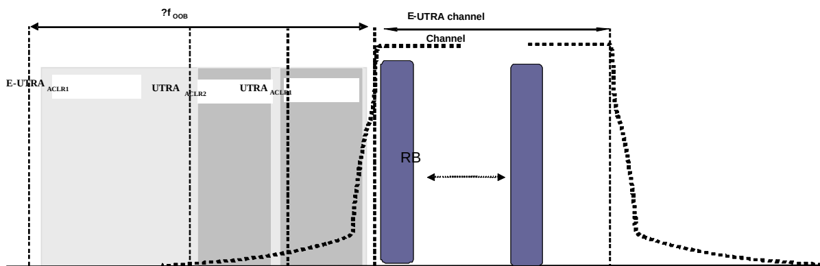
Figure 6.6.2B.3.1: Adjacent Channel Leakage Power Ratio requirements
