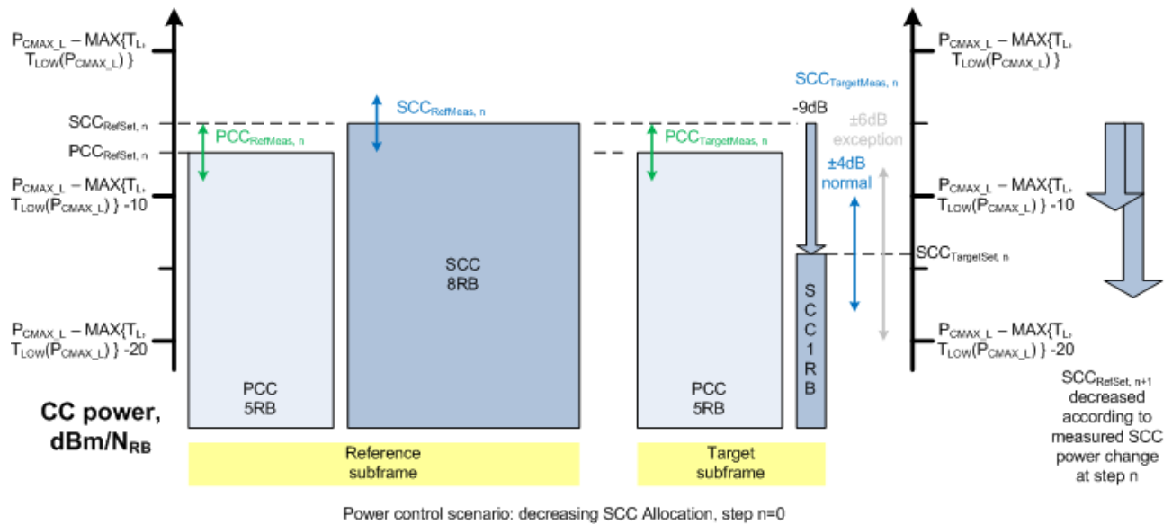
Figure 6.3.5A.2.1.4.2-2: SCC power decrease7. Sub test: PCC and SCC power increase together
