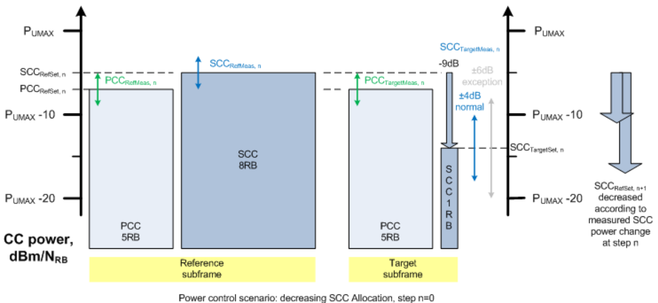
Figure 6.3.5A.2.1.4.2-2: SCC power decrease
