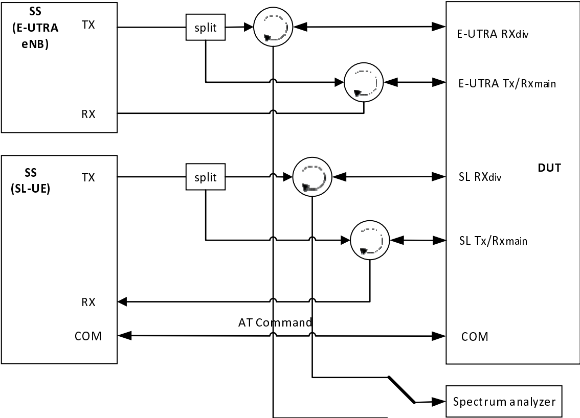
Figure A.93e: Connection for V2X Rx testing of simultaneous E-UTRA V2X sidelink and E-UTRA uplink transmission with additional Spectrum Analyzer
