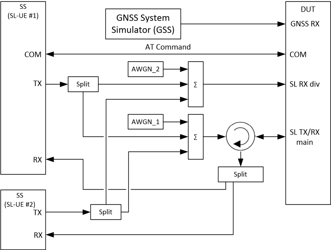
Figure A.98: Connection for power imbalance performance testing of V2V sidelink communications with two links in 1x2 AWGN channel and non-concurrent with E-UTRAN uplink transmission
