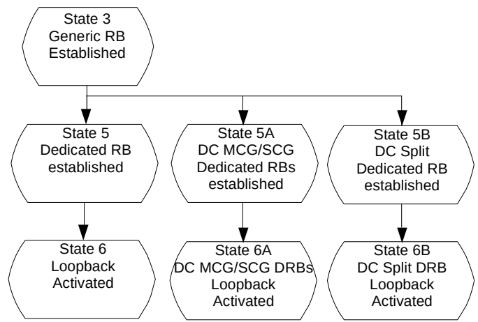
Figure 6.4.1.1-1: Initial UE states
