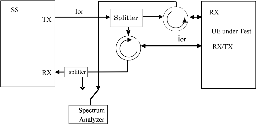
Figure A.8: Connection for RX-tests with additional Spectrum Analyzer
