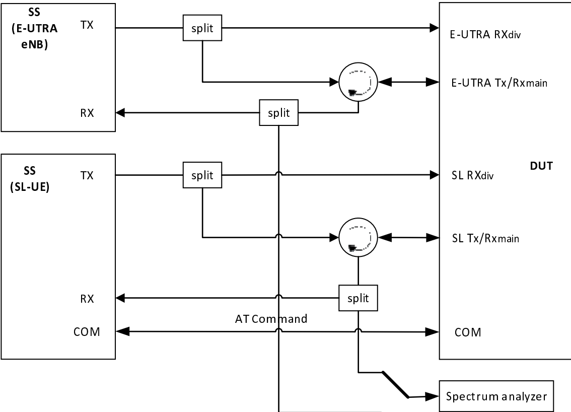
Figure A.93d: Connection for V2X Tx testing of simultaneous E-UTRA V2X sidelink and E-UTRA uplink transmission with additional Spectrum Analyzer
