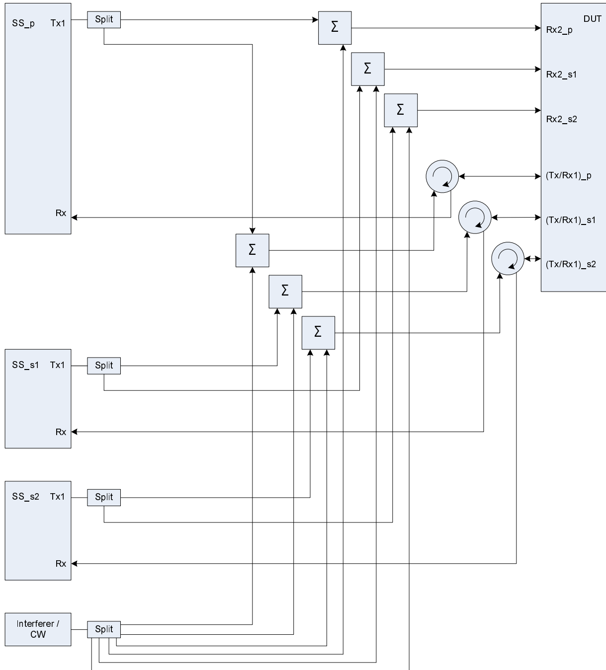
Figure A.58: Connection for Rx tests for CA (3CCs) with additional Interferer / CW
