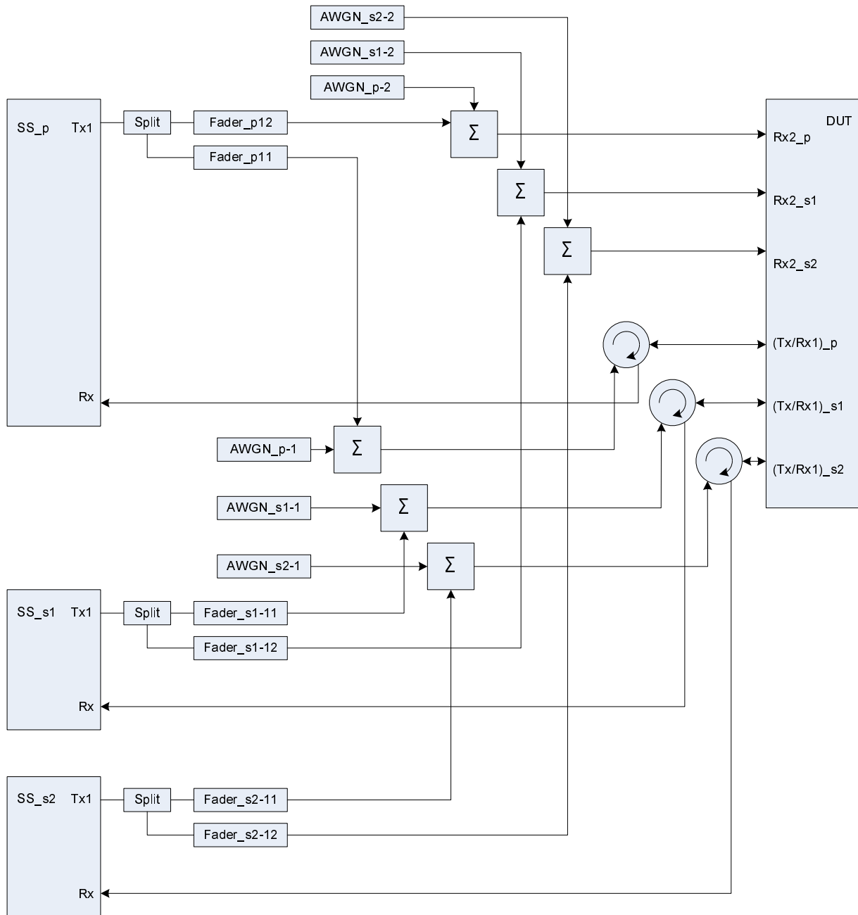
Figure A.59: Connection for Rx performance tests for CA (3CCs) with antenna configuration 1x2
