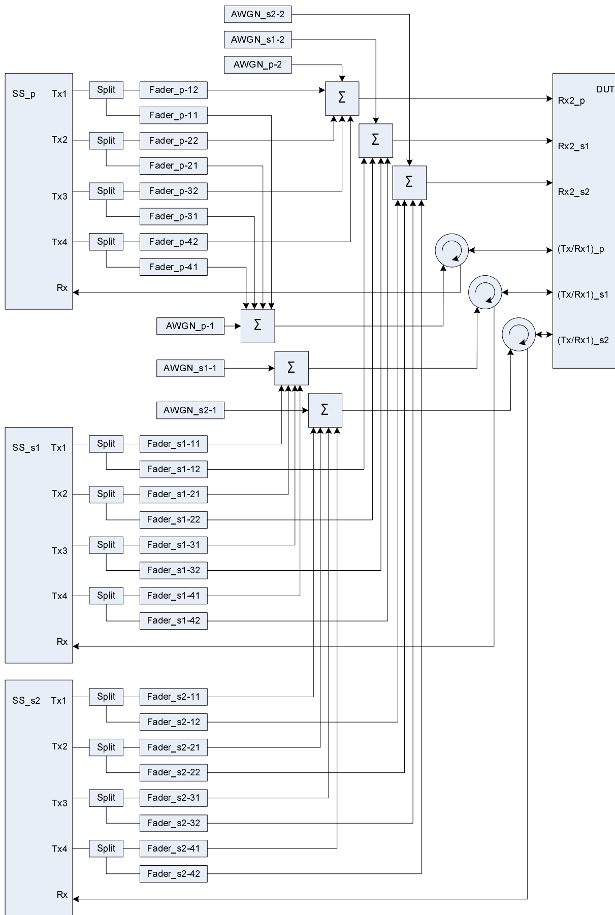
Figure A.61: Connection for Rx performance tests for CA (3CCs) with antenna configuration 4x2
