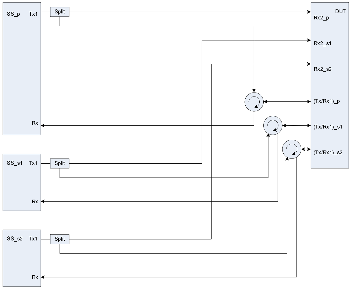
Figure A.55: Connection for basic Tx and Rx tests for CA (3CCs)
