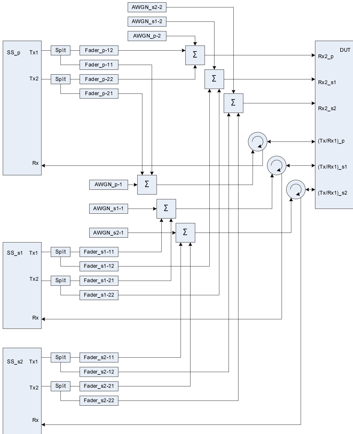
Figure A.60: Connection for Rx performance tests for CA (3CCs) with antenna configuration 2x2
