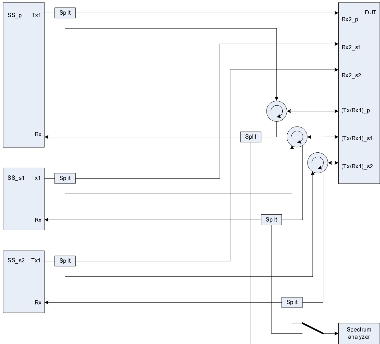
Figure A.56: Connection for Tx tests for CA (3CCs) with additional Spectrum Analyzer
