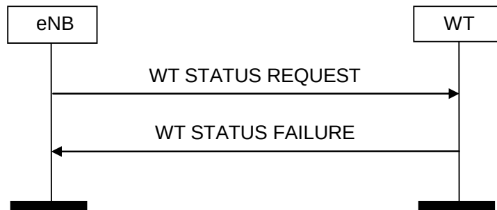
Figure 8.4.3-1: WT Status Reporting Initiation procedure, unsuccessful operation
