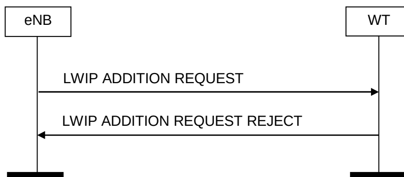
Figure 8.14.3-1: LWIP Addition Preparation, unsuccessful operation
