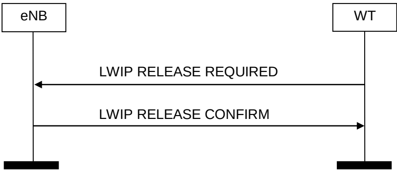
Figure 8.17.2-1: WT initiated LWIP Release, successful operation
