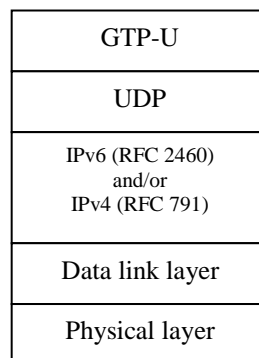
Figure 6.1: Transport network layer for data streams over X2
