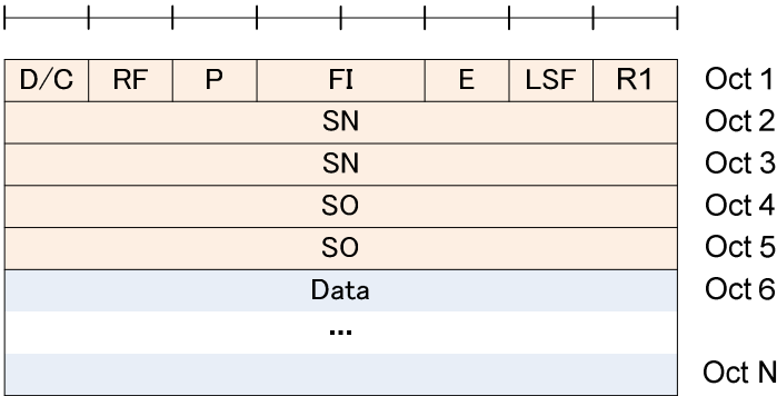
Figure 6.2.1.5-1a: AMD PDU segment with 16 bit SN and with 16 bit SO (No LI)
