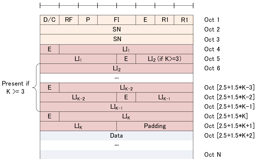
Figure 6.2.1.4-2a: AMD PDU with 16 bit SN (length of LI field is 11 bits) (Odd number of LIs, i.e. K = 1, 3, 5, ...)
