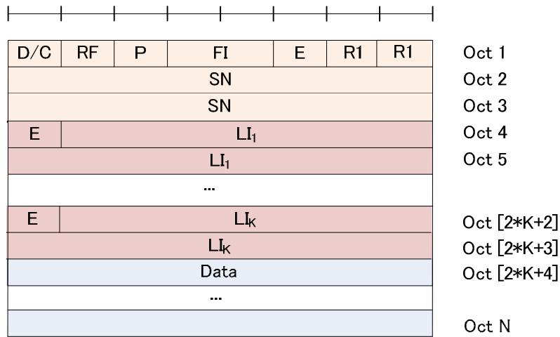
Figure 6.2.1.4-a: AMD PDU with 16 bit SN (length of LI field is 15 bits)
