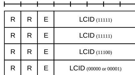
Case 4: MAC subheader for two-byte padding + MAC subheader for MAC control element + MAC subheader for MAC SDU (CCCH or DCCH)
