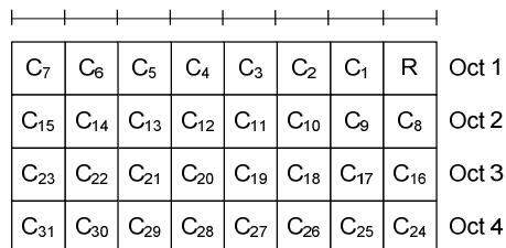
Figure 6.1.3.15-2: Hibernation MAC control element of four octets
