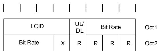
Figure 6.1.3.13-1: Recommended bit rate MAC control element
