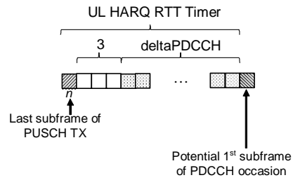
Figure C-2: Setting the UL HARQ RTT Timer for NB-IoT
