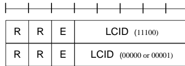
Case 2: MAC subheader for MAC control element + MAC subheader for MAC SDU (CCCH or DCCH)
