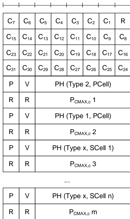
Figure 6.1.3.6a2-4: Extended PHR MAC Control Element supporting 32 serving cells with configured uplink
