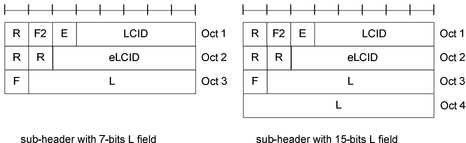
Figure 6.1.2-1: R/F2/E/LCID/(R/R/eLCID)/F/L MAC subheader with 7-bits and 15-bits L field
