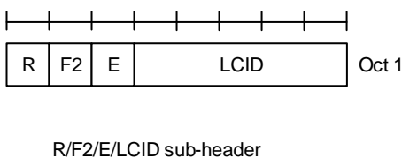
Figure 6.1.2-2: R/F2/E/LCID MAC subheader
