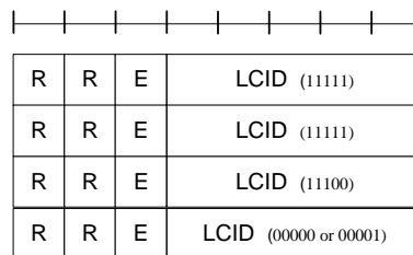
Case 4: MAC subheaders for two-byte padding + MAC subheader for MAC control element + MAC subheader for MAC SDU (CCCH or DCCH)
