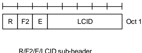
Figure 6.1.2-2: R/F2/E/LCID MAC subheader
