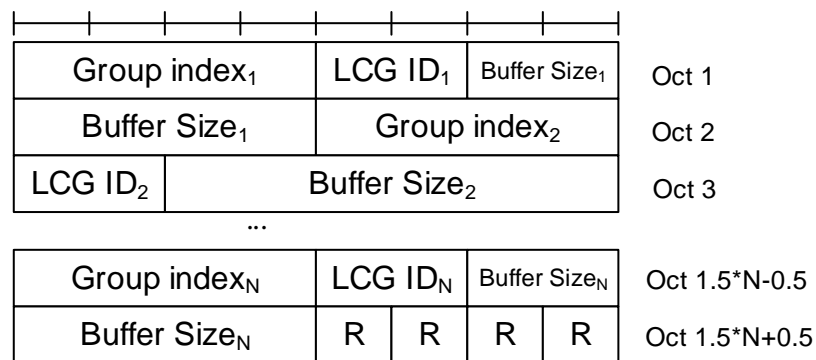
Figure 6.1.3.1a-2: Sidelink BSR MAC control element for odd N
