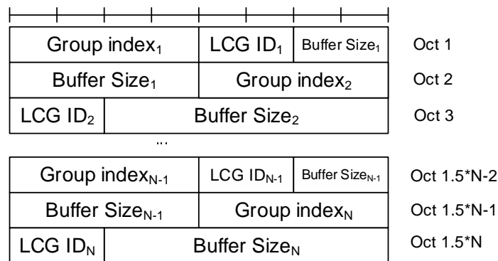
Figure 6.1.3.1a-1: Sidelink BSR MAC control element for even N
