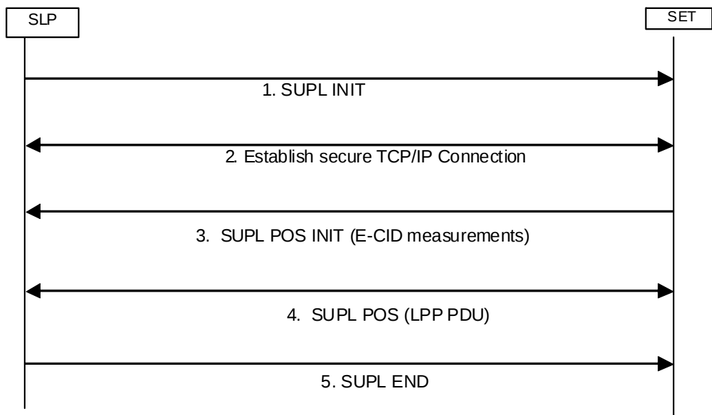
Figure B.3-1: LPP session over SUPL
