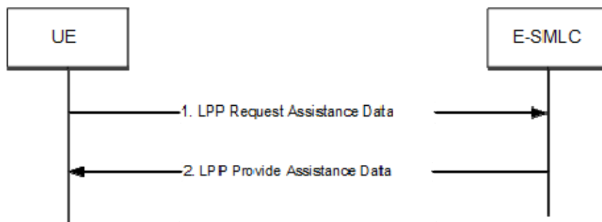
Figure 8.8.3.3.2-1: UE-initiated Assistance Data Transfer Procedure
