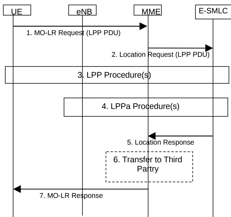
Figure 7.3.2-1: UE Positioning Operations to support an MO-LR
