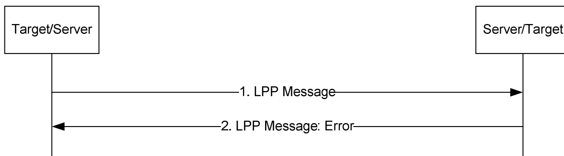
Figure 7.1.2.6-1: Error handling
