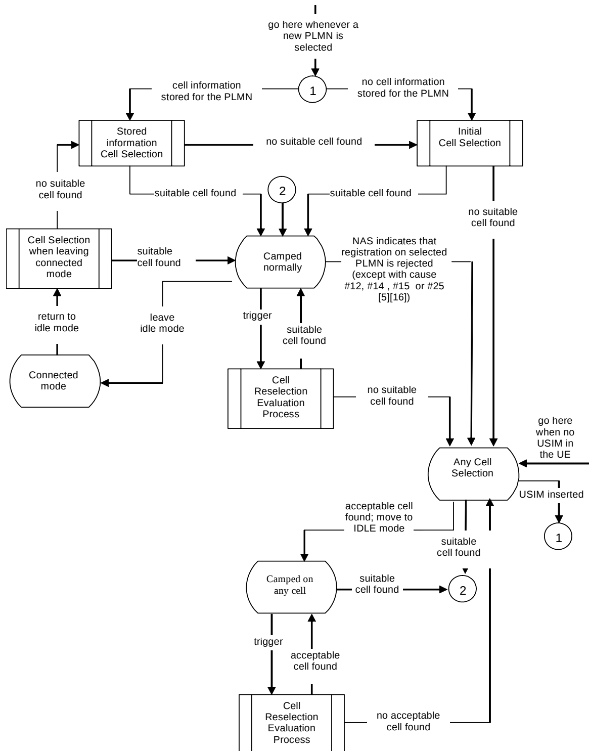
Figure 5.2.2-2: RRC_IDLE Cell Selection and Reselection for NB-IoT
