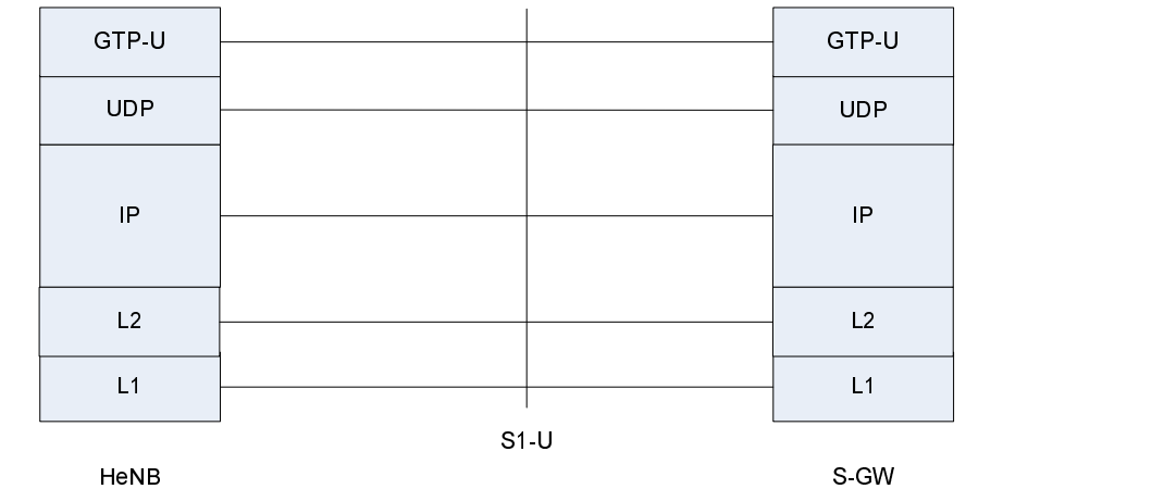
Figure 4.6.3.1-1: User plane for S1-U interface for HeNB without HeNB GW
