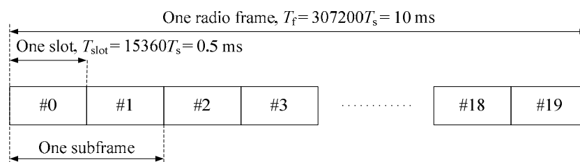
Figure 4.1-1: Frame structure type 1 (assuming \Delta f \in \{2.5, 7.5, 15\} kHz).
