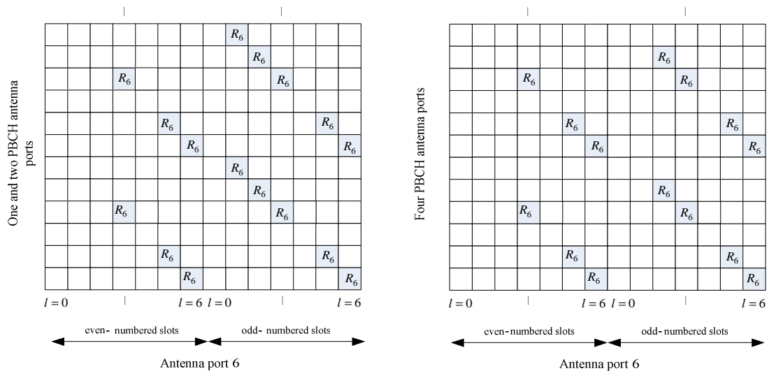
Figure 6.10.4.2-1: Mapping of positioning reference signals (normal cyclic prefix)
