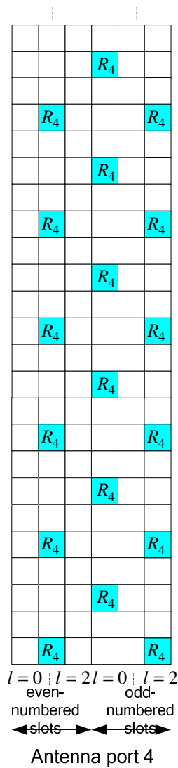
Figure 6.10.2.2-3: Mapping of MBSFN reference signals (extended cyclic prefix, \Delta f = 7.5\text{kHz} )
