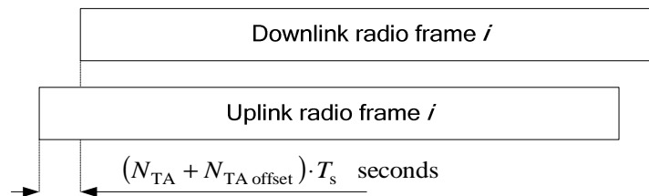
Figure 8.1-1: Uplink-downlink timing relation
