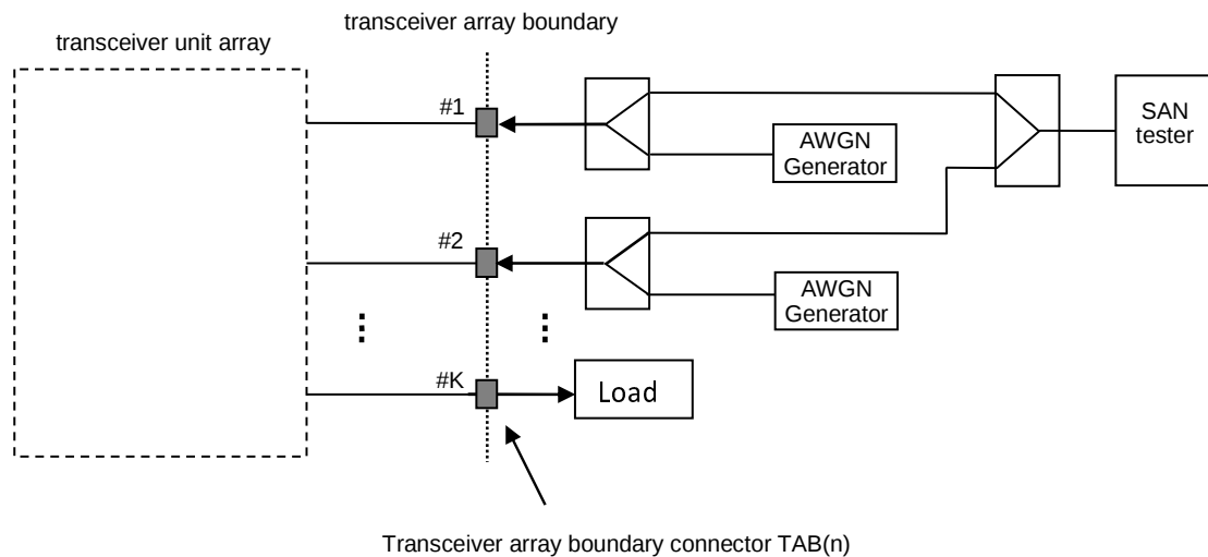
Figure D.5.2-2: Functional set-up for performance requirements for PUSCH and PRACH in static conditions for SAN with Rx diversity (2 Rx case shown)
