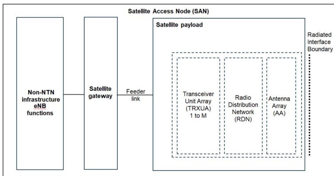
Figure 4.2.2-1: Radiated reference points for SAN type 1-O
