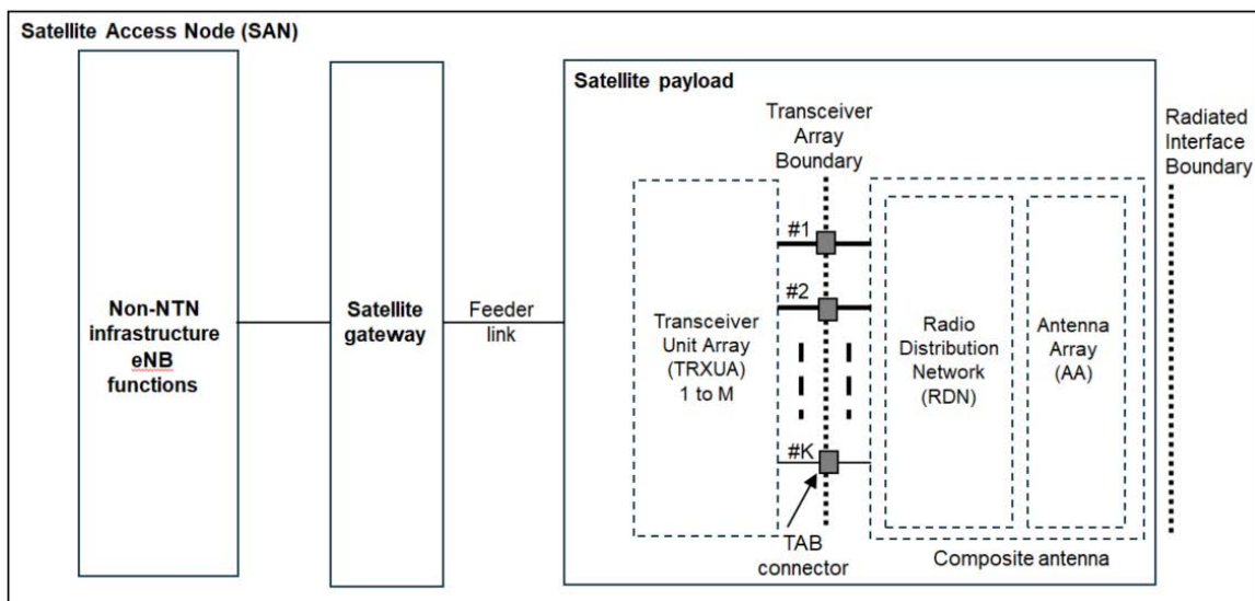
Figure 4.2.1-1: Radiated and conducted reference points for SAN type 1-H
