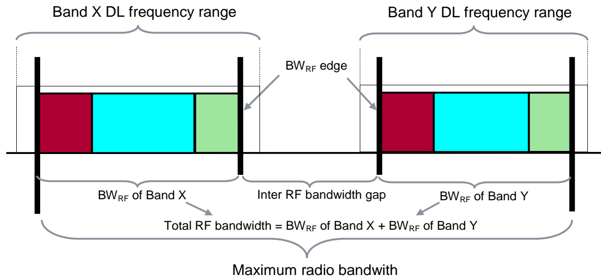
Figure 3.2-1 Illustration of Maximum Radio Bandwidth BW_{\text{max}} and Total RF Bandwidth BW_{\text{tot}} for multi-band base station
